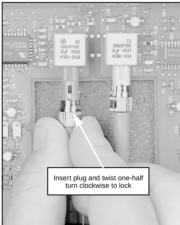
Figure 18 Glass fiber-optic cable connections on the Fiber Receiver card
