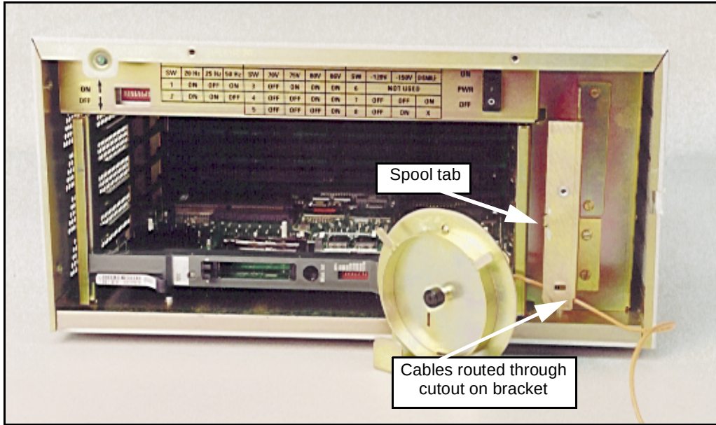
Figure 20 Fiber routing bracket installed in the Main chassis.
