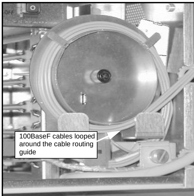
Figure 26 100BaseF cables looped around the cable routing guide on the front of the chassis
