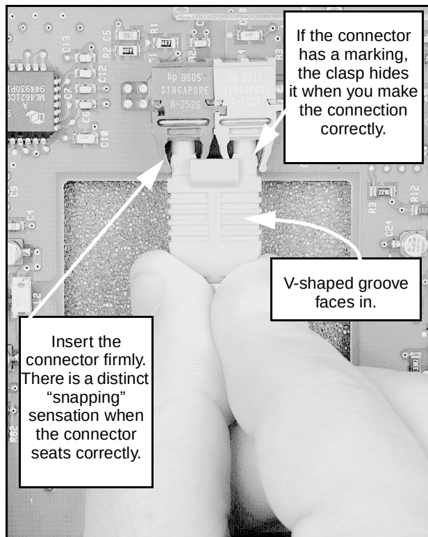
Figure 16 Plastic fiber-optic cable connections on the Fiber Receiver card
