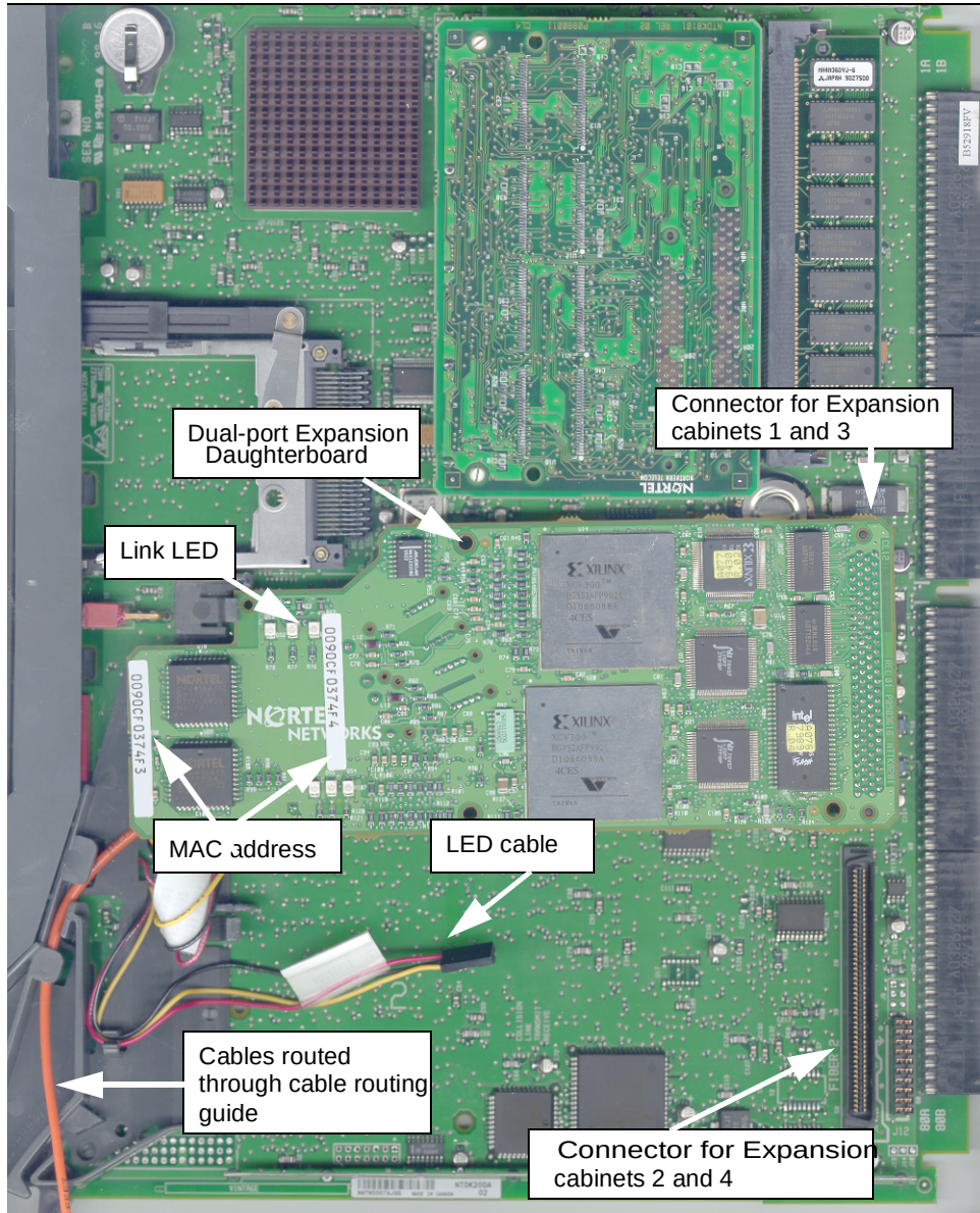
Figure 24 SSC card for the Main chassis
