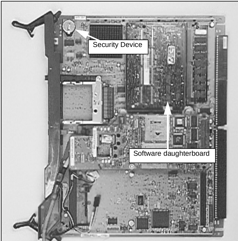
Figure 25 Software daughterboard on the SSC card
