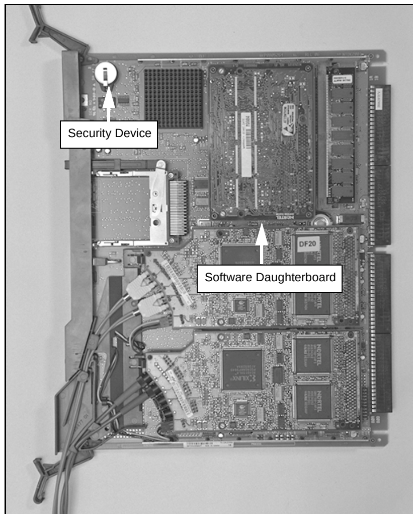
Figure 9 Security Device and Software Daughterboard on the SSC card
