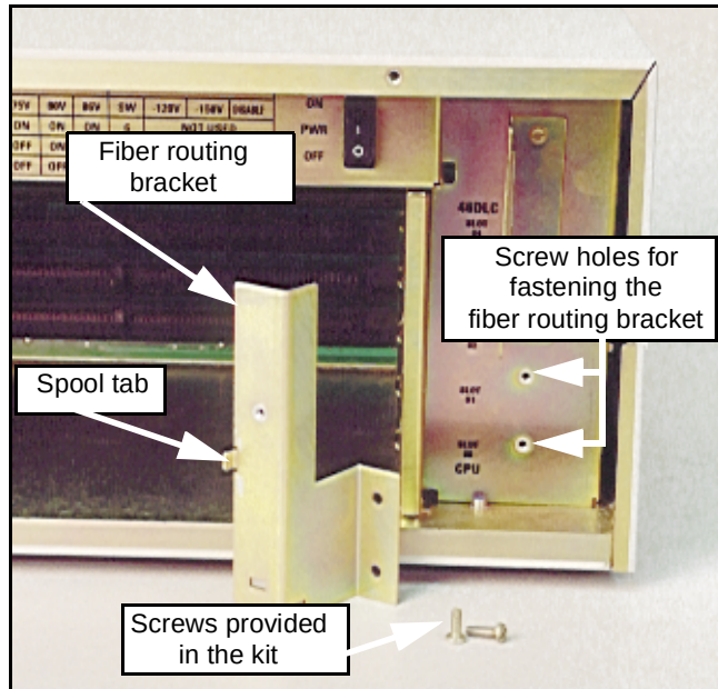
Figure 19 Fiber routing bracket
