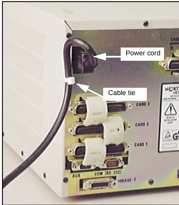
Figure 30 Power connector on the back of the chassis
