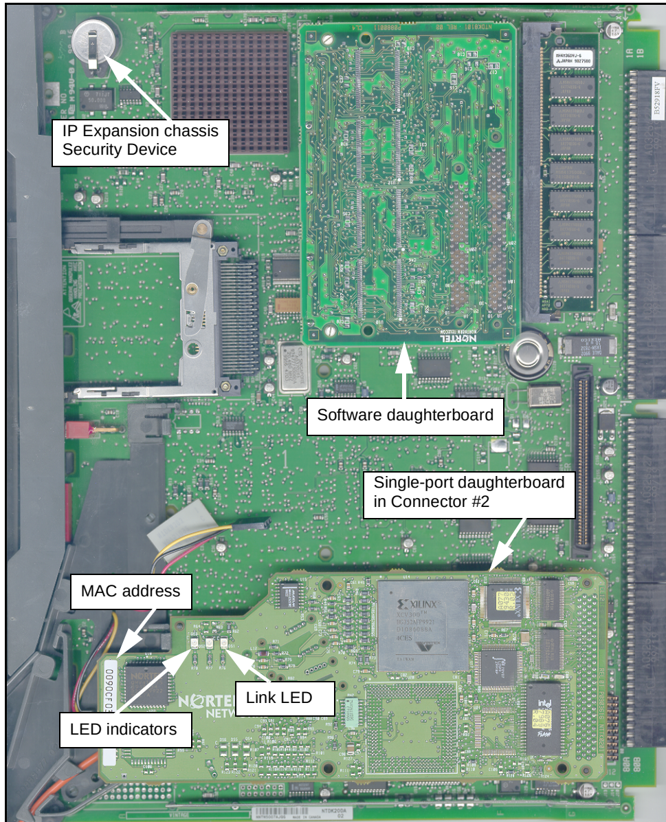
Figure 29 SSC card for the Expansion chassis
