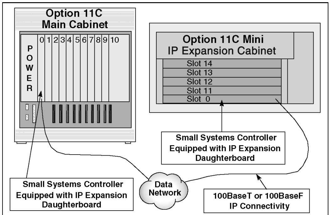
Figure 5 Option 11C and Option 11C Mini IP expansion configuration
