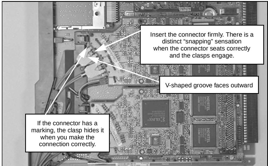
Figure 10 Plastic fiber-optic cable connection on the SSC card
