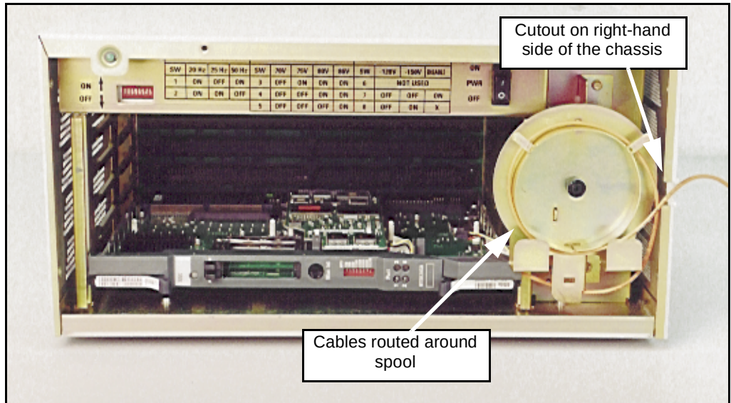
Figure 21 Fiber routing guide installed in the chassis
