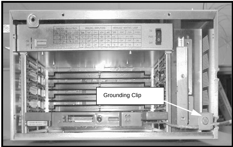
Figure 7 Option 11C Mini EMC grounding clip location
