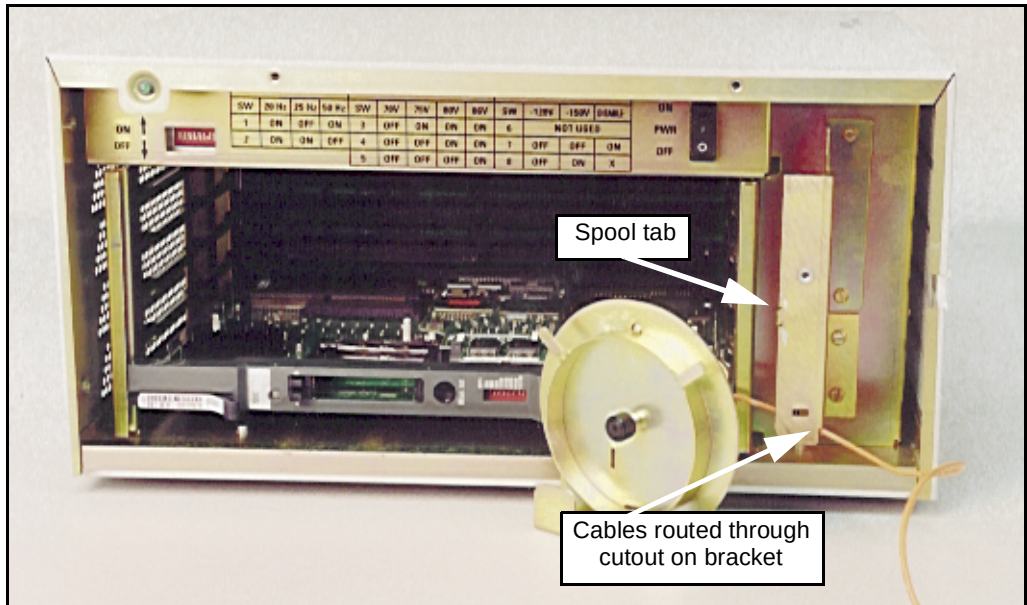
Figure 14 Fiber routing bracket installed on the chassis
