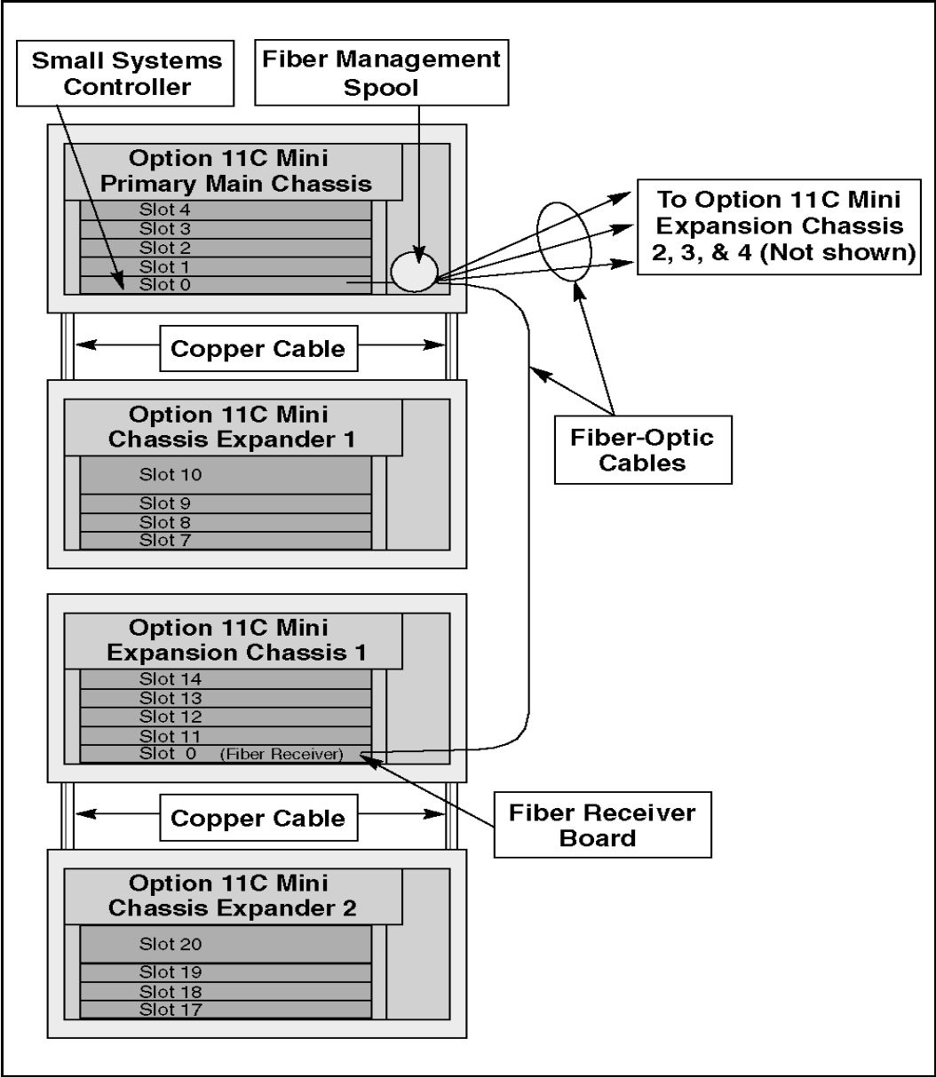
Figure 4 Option 11C Mini fiber-optic expansion configuration including Chassis Expander.
