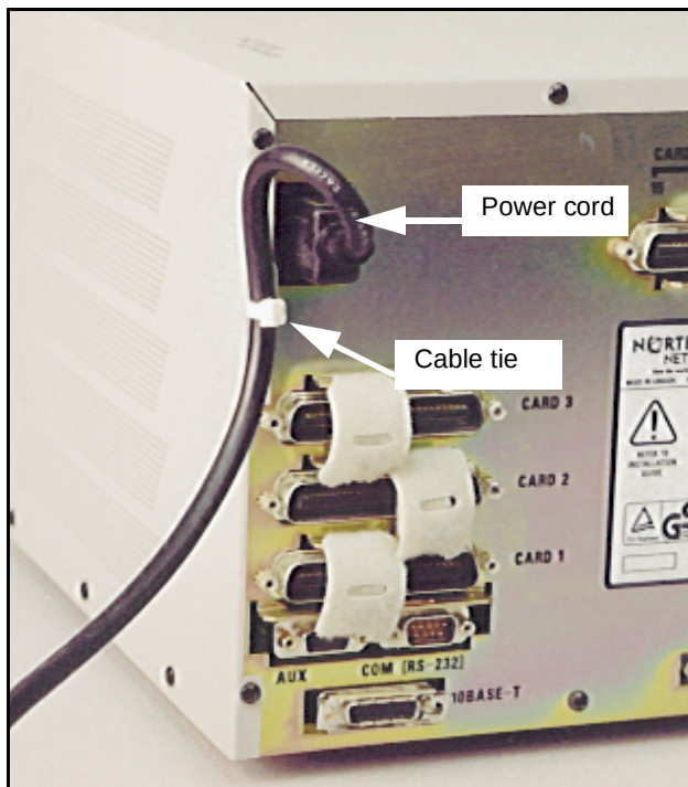
Figure 22 Power connector on the back of the chassis
