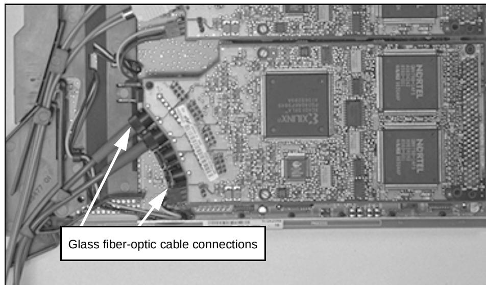
Figure 11 Glass fiber-optic cable connection on the SSC card
