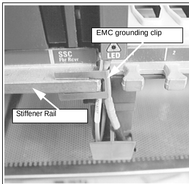
Figure 6 Option 11C EMC grounding clip
