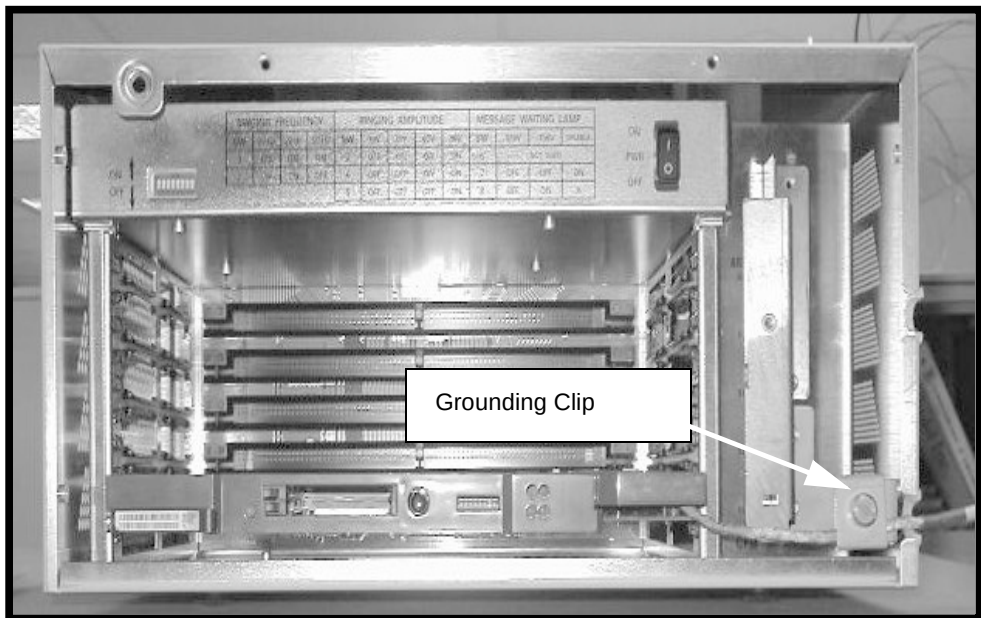
Figure 27 EMC grounding clip location
