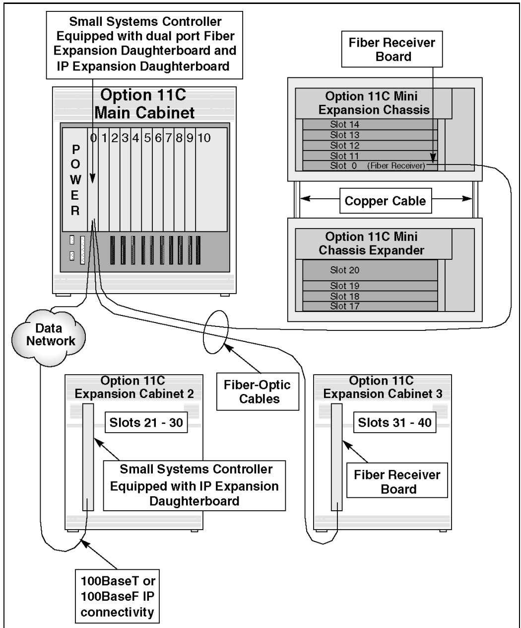
Figure 8 Option 11C and Option 11C Mini mix-and-match expansion configuration
