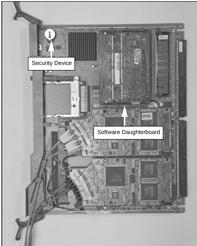
Figure 23 Security Device and Software Daughterboard on the SSC card
