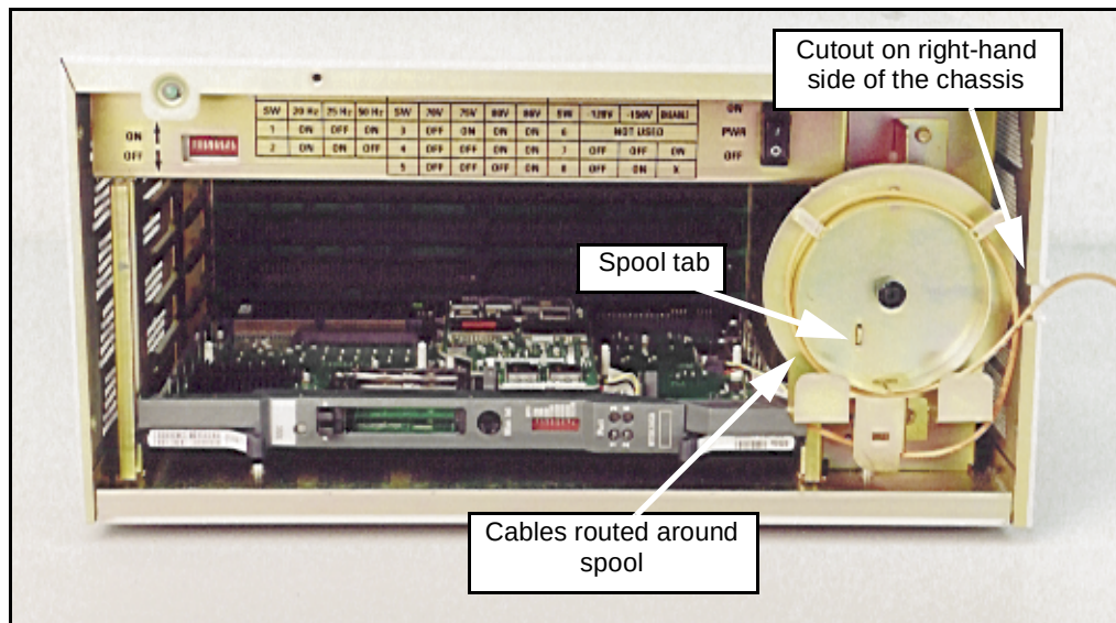
Figure 15 Fiber routing guide installed in the chassis
