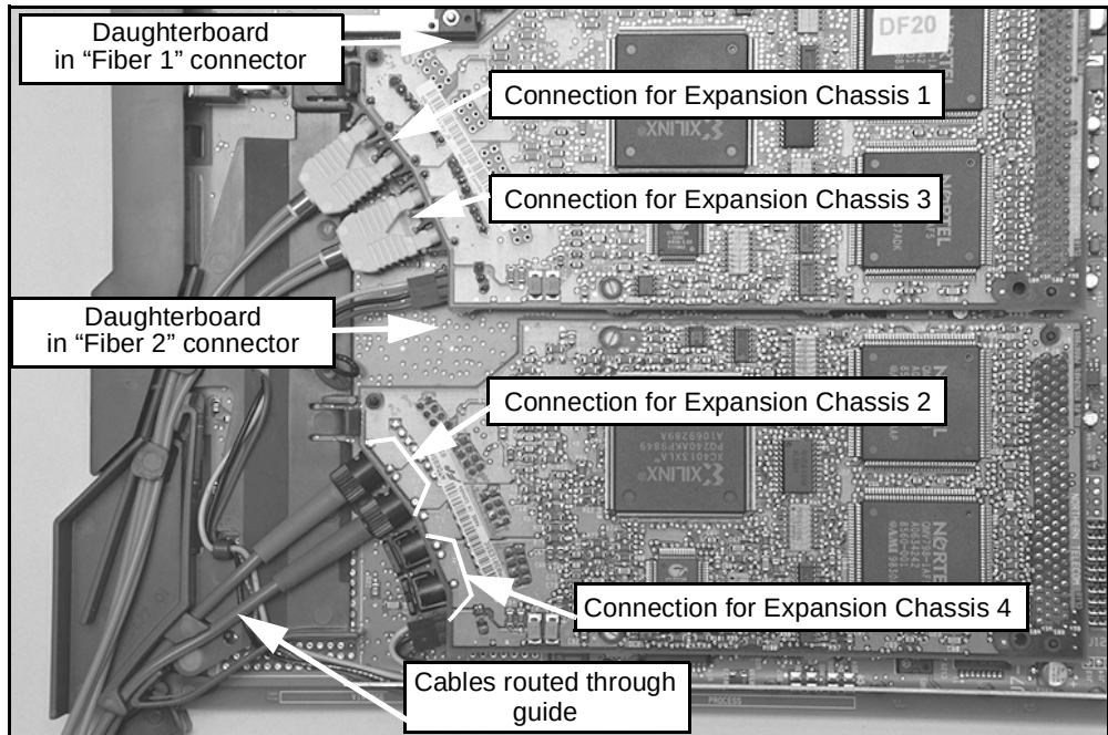
Figure 12 Daughterboard connectors on the SSC card
