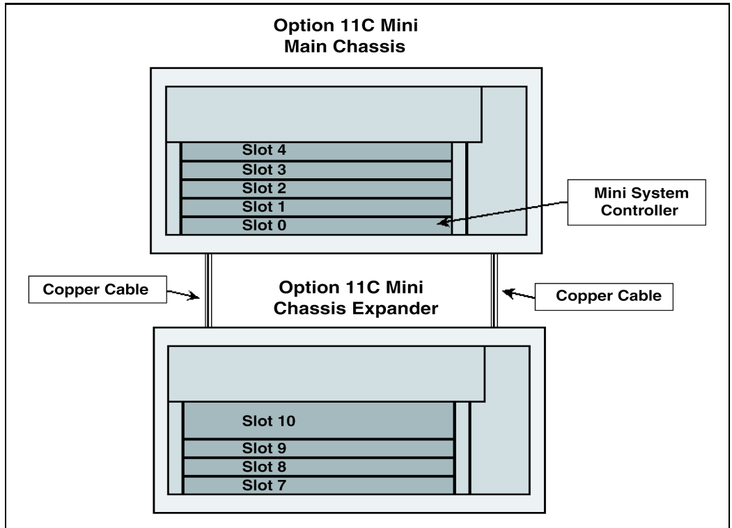
Figure 2 Option 11C Mini Main Chassis connected to a Chassis Expander
