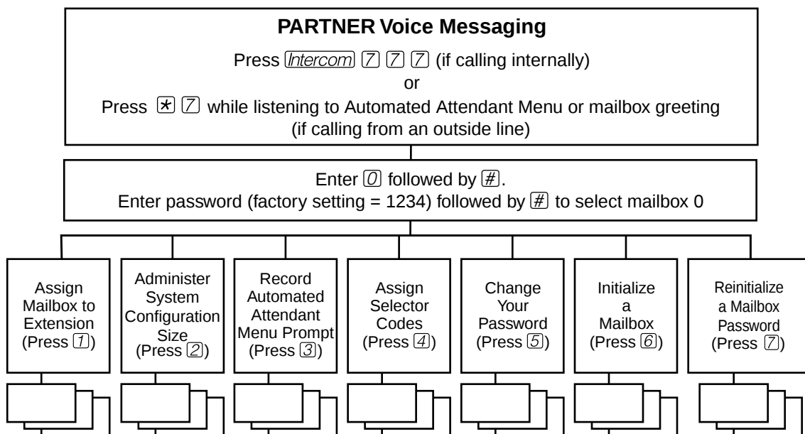
Figure 3. System Administration Menu
